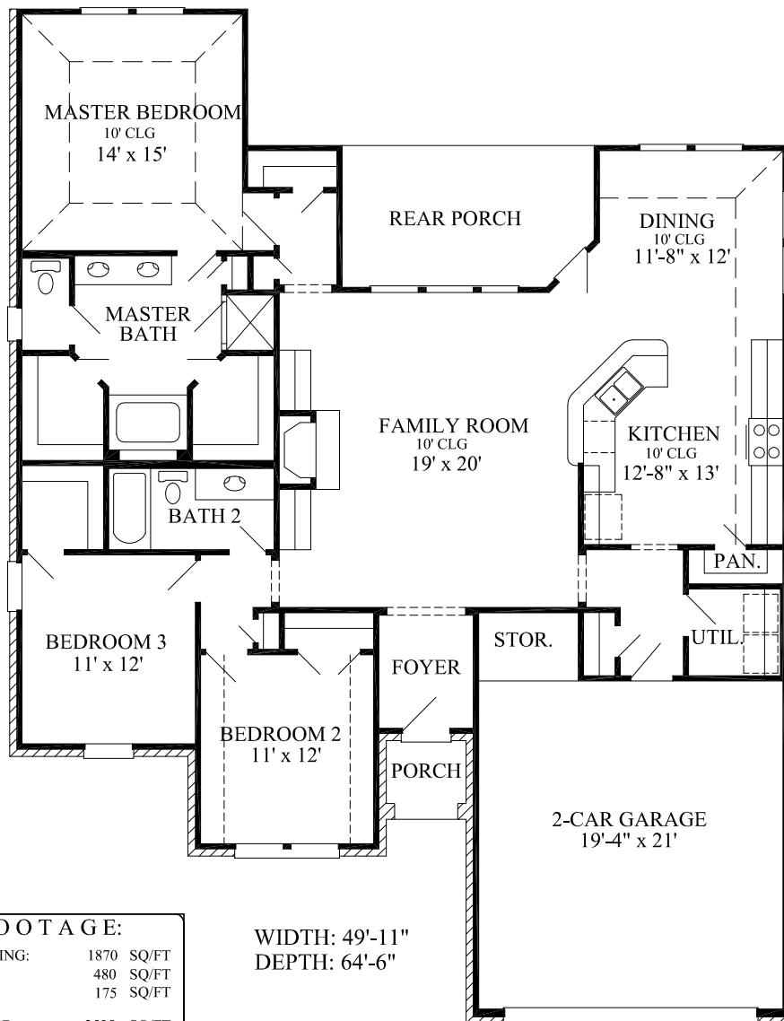
FLOOR PLAN
