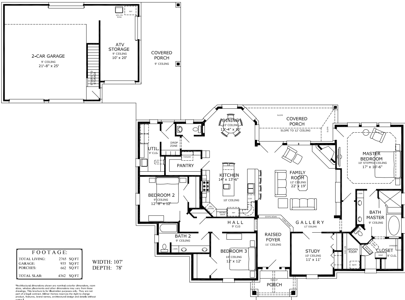
FLOOR PLAN
