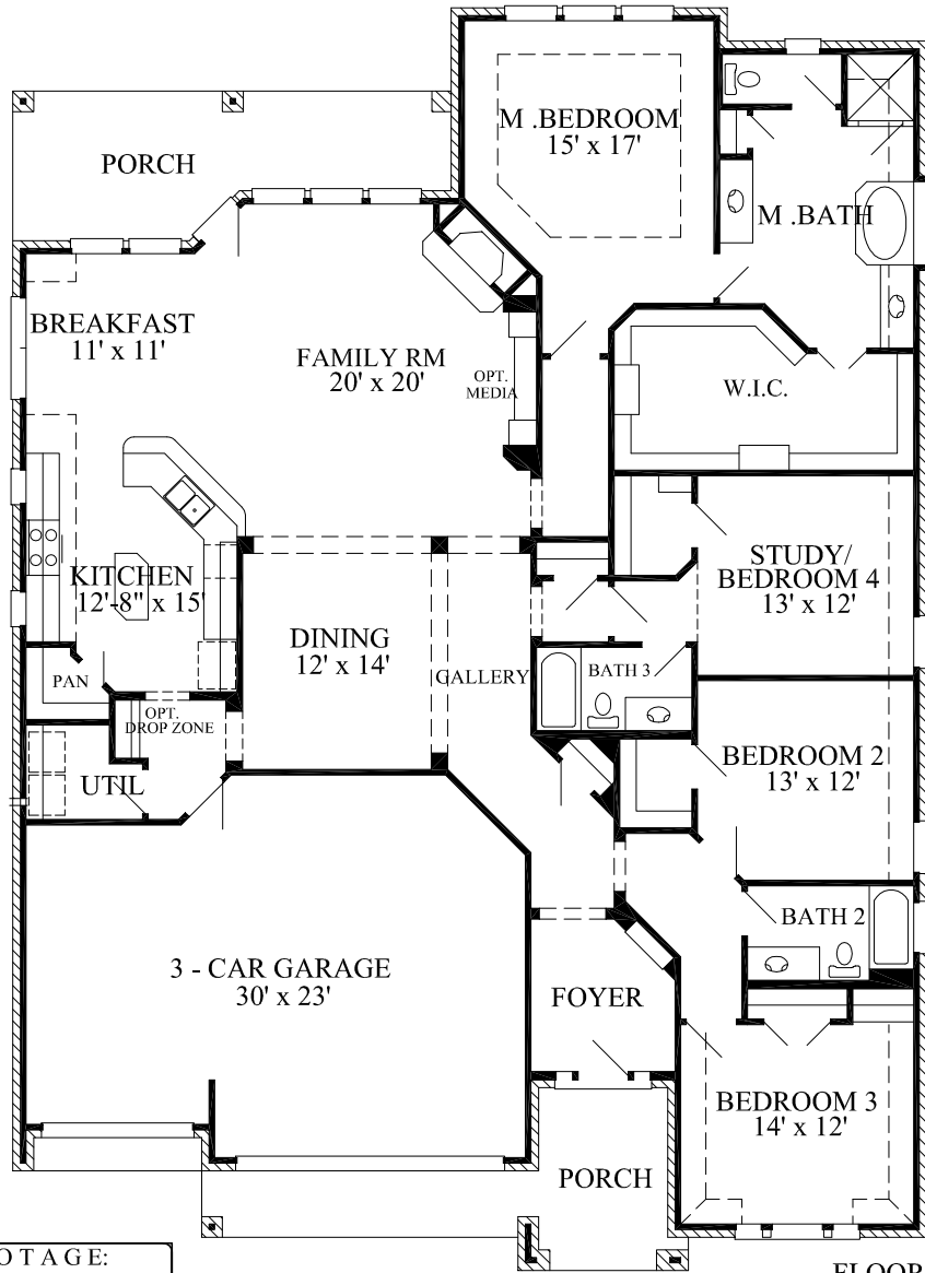
FLOOR PLAN
