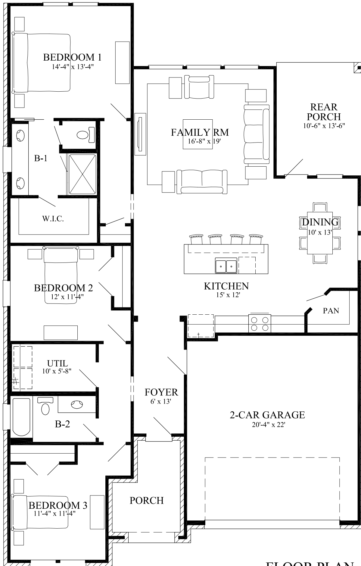
FLOOR PLAN
