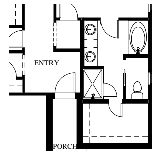
MASTER BATH WITH GARDEN TUB AND SHOWER
